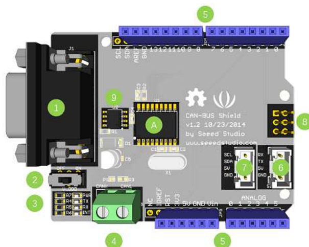
Figure -9- Carte CAN-BUS, face avant ( CAN-BUS Shield V1.2 | Sees Studio Wiki ).
